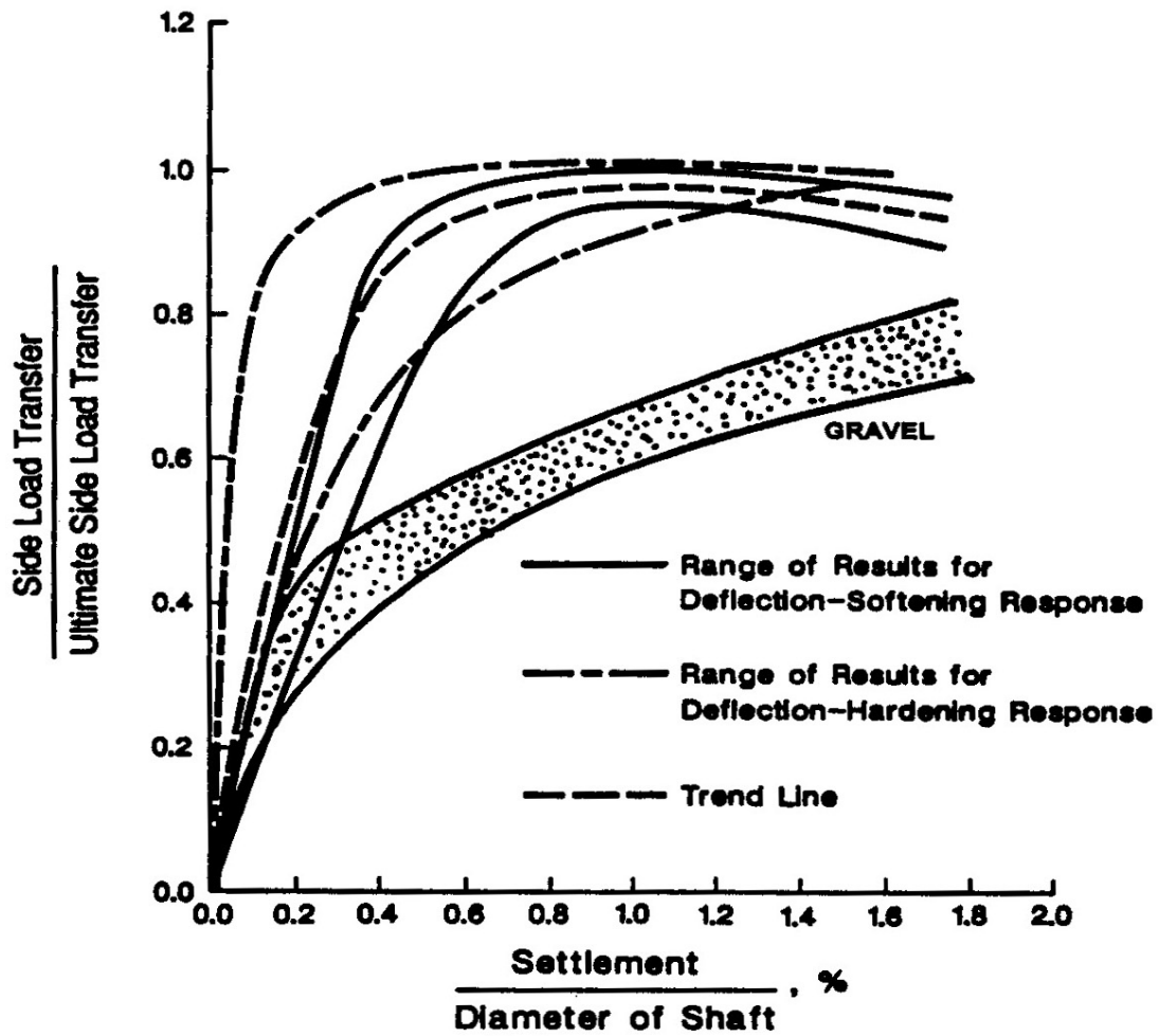
Figure 1: Normalized Side Load Transfer Curves for Drilled Shafts in Cohesionless Soils (Figure 10.8.2.2.2-3 of AASHTO (2007)).
