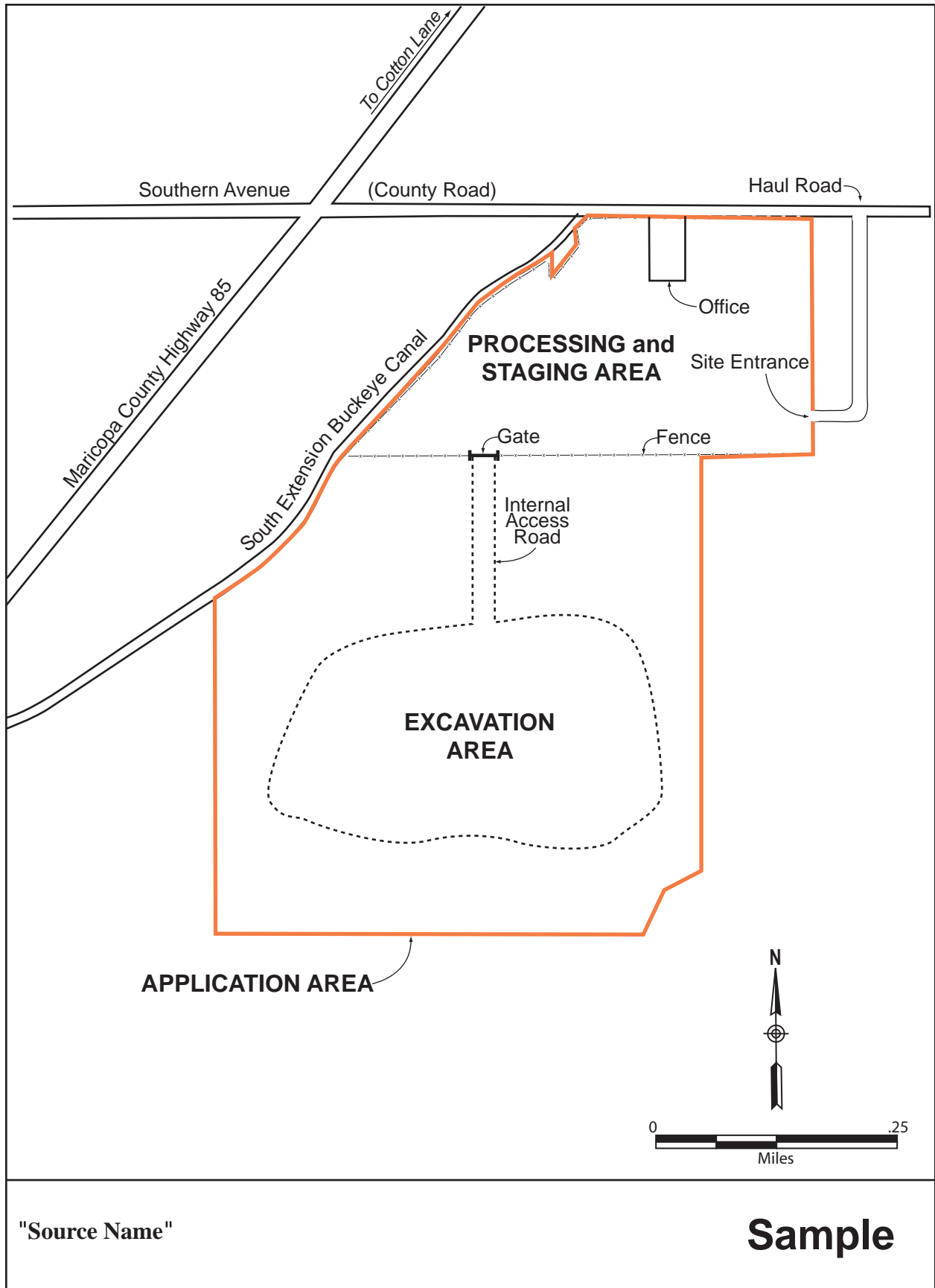
Figure 3. Site Plan
