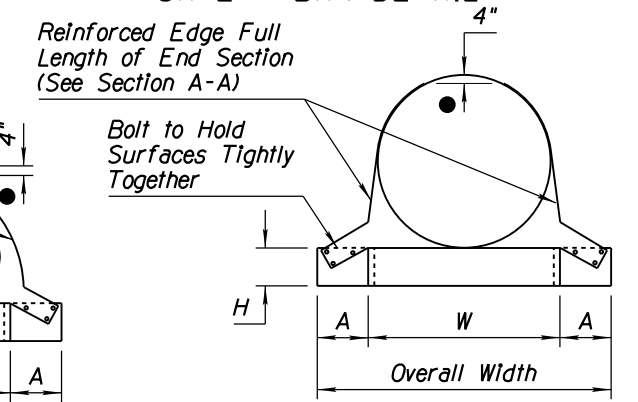
FRONT VIEW-ROUND PIPE
