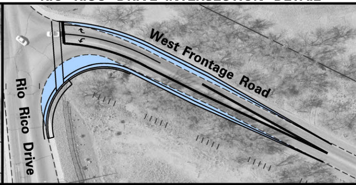
WEST FRONTAGE ROAD AND RIO RICO DRIVE INTERSECTION DETAIL
