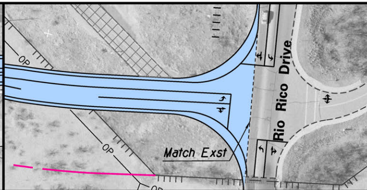
RIO RICO DRIVE INTERSECTION DETAIL
