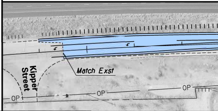
KIPPER STREET INTERSECTION DETAIL
