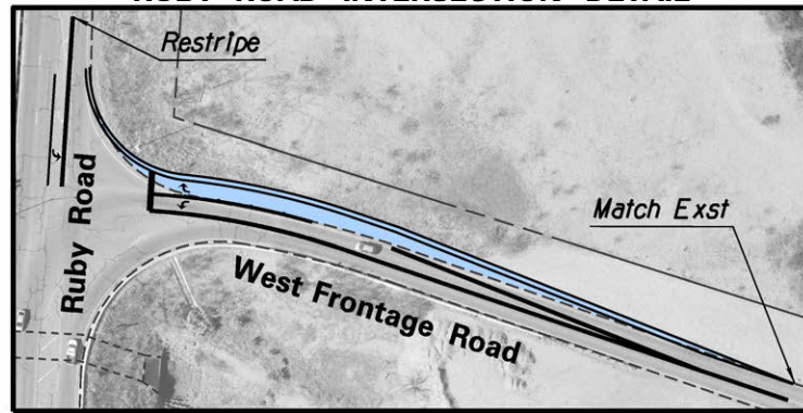
WEST FRONTAGE ROAD AND RUBY ROAD INTERSECTION DETAIL
