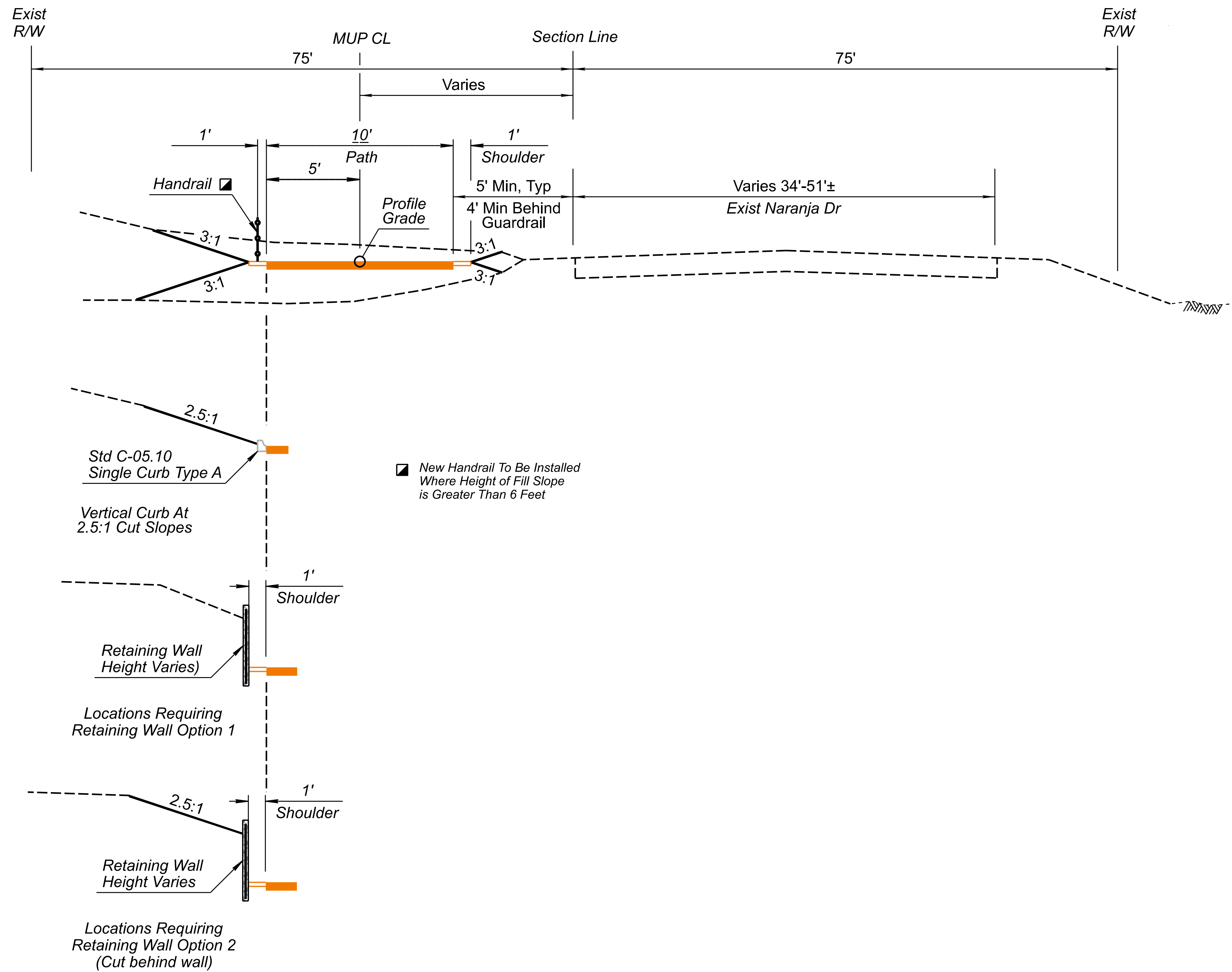
MULTI-USE PATH TYPICAL SECTION
