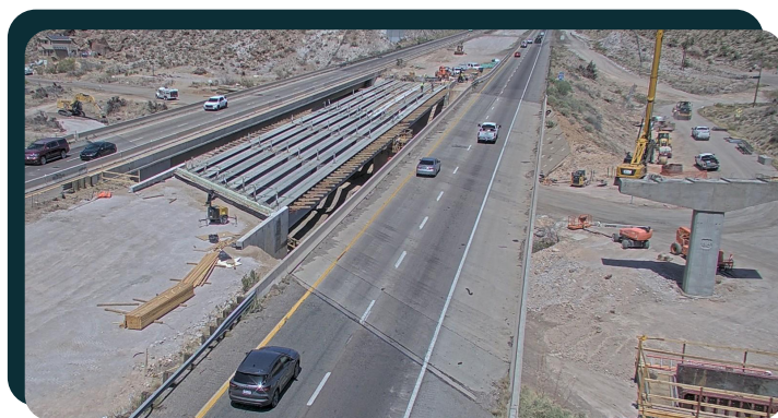
Clack Canyon Road Bridge after the girder installation work was completed.
