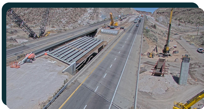
After the second night of girder installation work.
