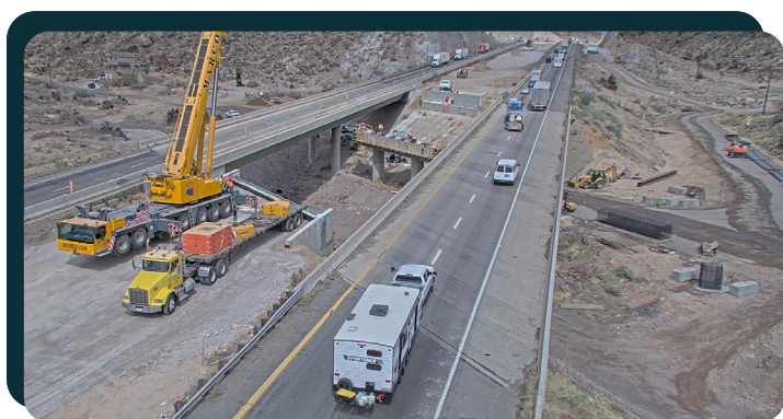
Clack Canyon Road Bridge prior to the girders being installed.
