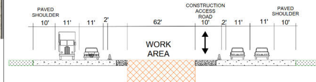
I-10 TYPICAL SECTION PHASE 2
