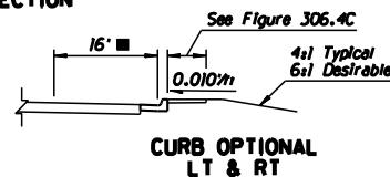
URBAN HIGHWAY TYPICAL SECTIONS FIGURE 306.4A
