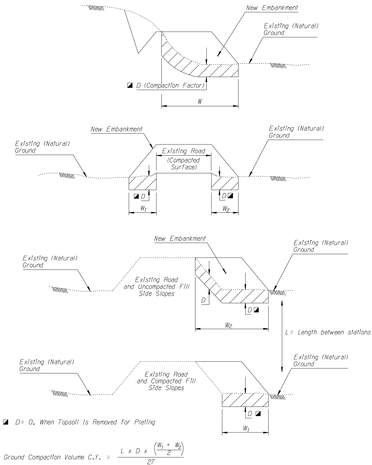
GROUND COMPACTION APPLICATIONS FIGURE 701.4C
