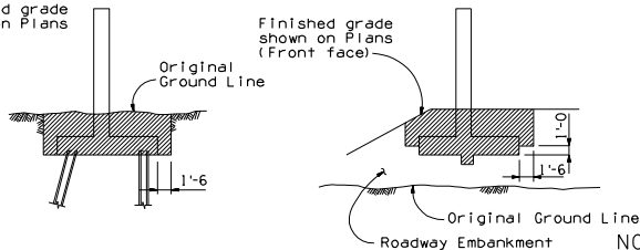
TYPICAL RETAINING WALL SECTIONS
