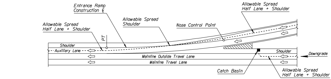
Urban 1 - Lane Entrance Ramp Parallel Type With Auxiliary Lane
