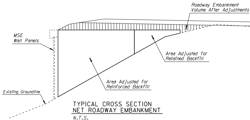
TYPICAL CROSS SECTION ROADWAY EMBANKMENT & ADJUSTMENTS N.T.S.
