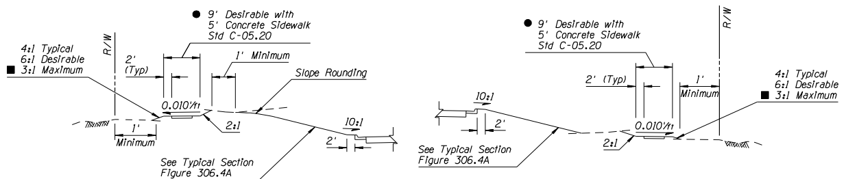
SIDEWALK LOCATION WITH LIMITED R/W
