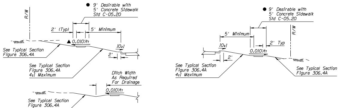
OPTIONAL SIDEWALK LOCATION
