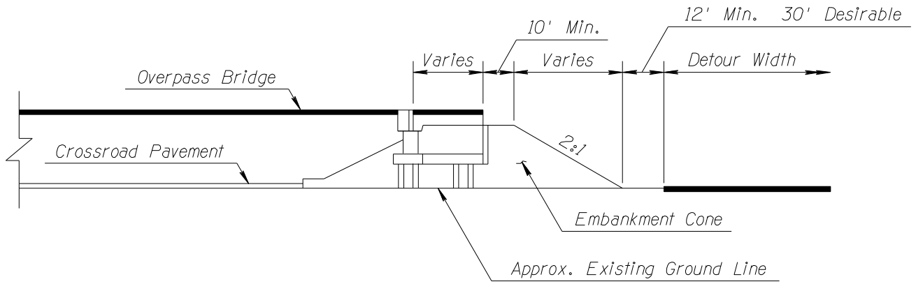
Embankment Condition
