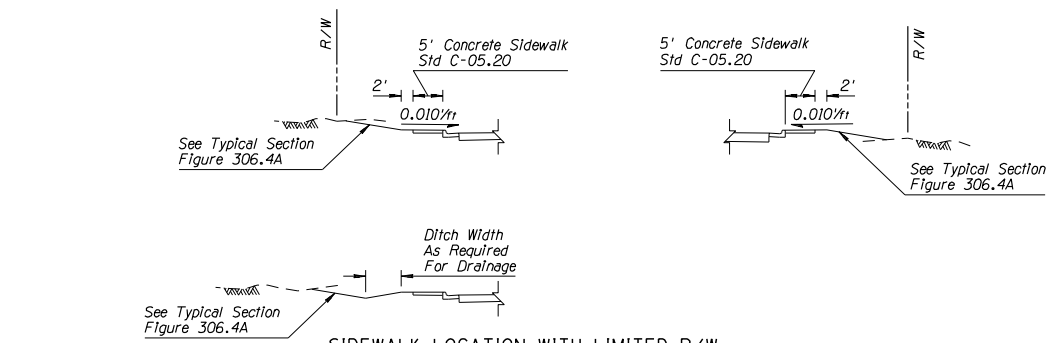
SIDEWALK LOCATION WITH LIMITED R/W
