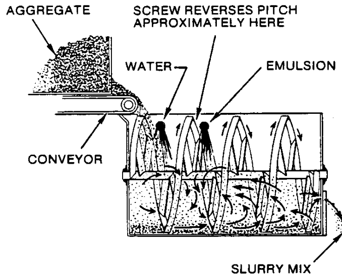
Figure A Flow diagram of slurry mixer
