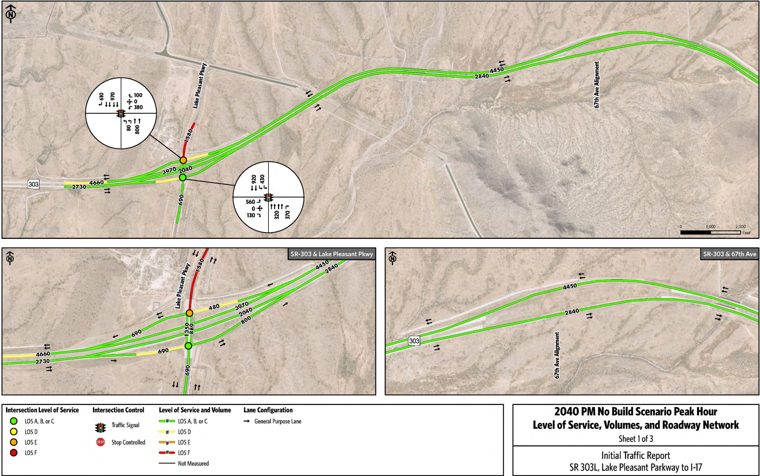
Figure 4-13: Year 2040 No Build Peak Hour PM - Traffic Volumes, Lanes, & LOS (Sheet 1 of 3)
