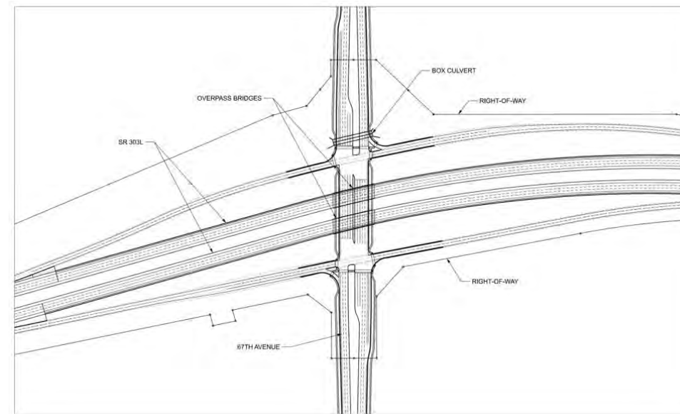
Figure 4-7: Diamond Interchange
