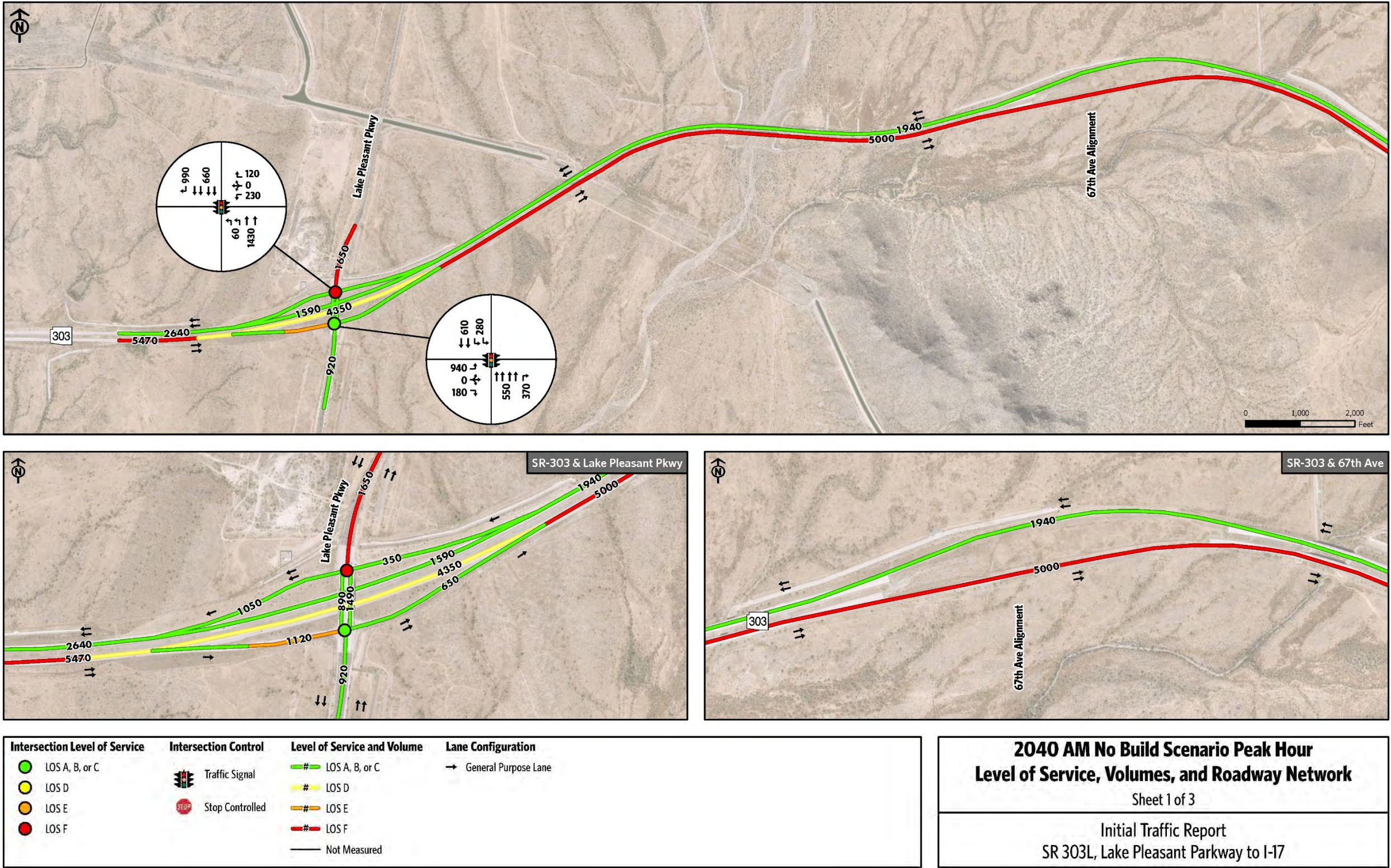
Figure 4-10: Year 2040 No Build AM Peak Hour - Traffic Volumes, Lanes, & LOS (Sheet 1 of 3)
