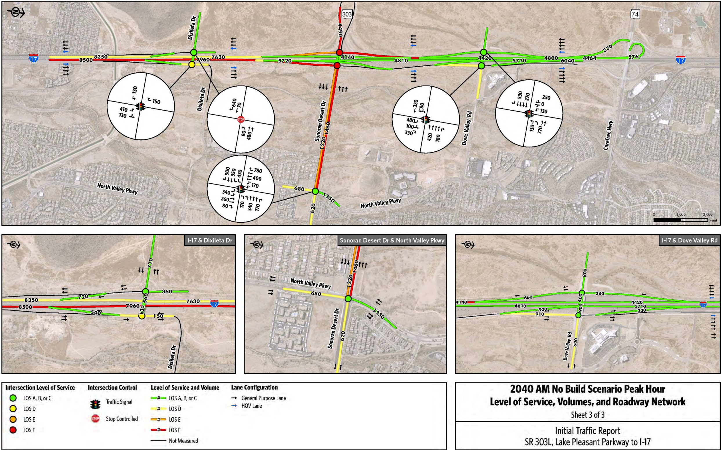
Figure 4-12: Year 2040 No Build AM Peak Hour - Traffic Volumes, Lanes, & LOS (Sheet 3 of 3)
