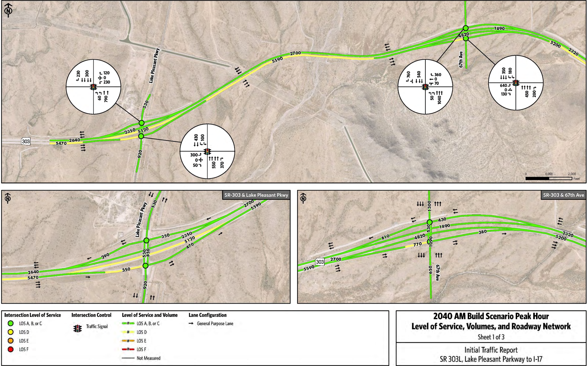
Figure 4-16: Year 2040 Build AM Peak Hour - Traffic Volumes, Lanes, & LOS (Sheet 1 of 3)
