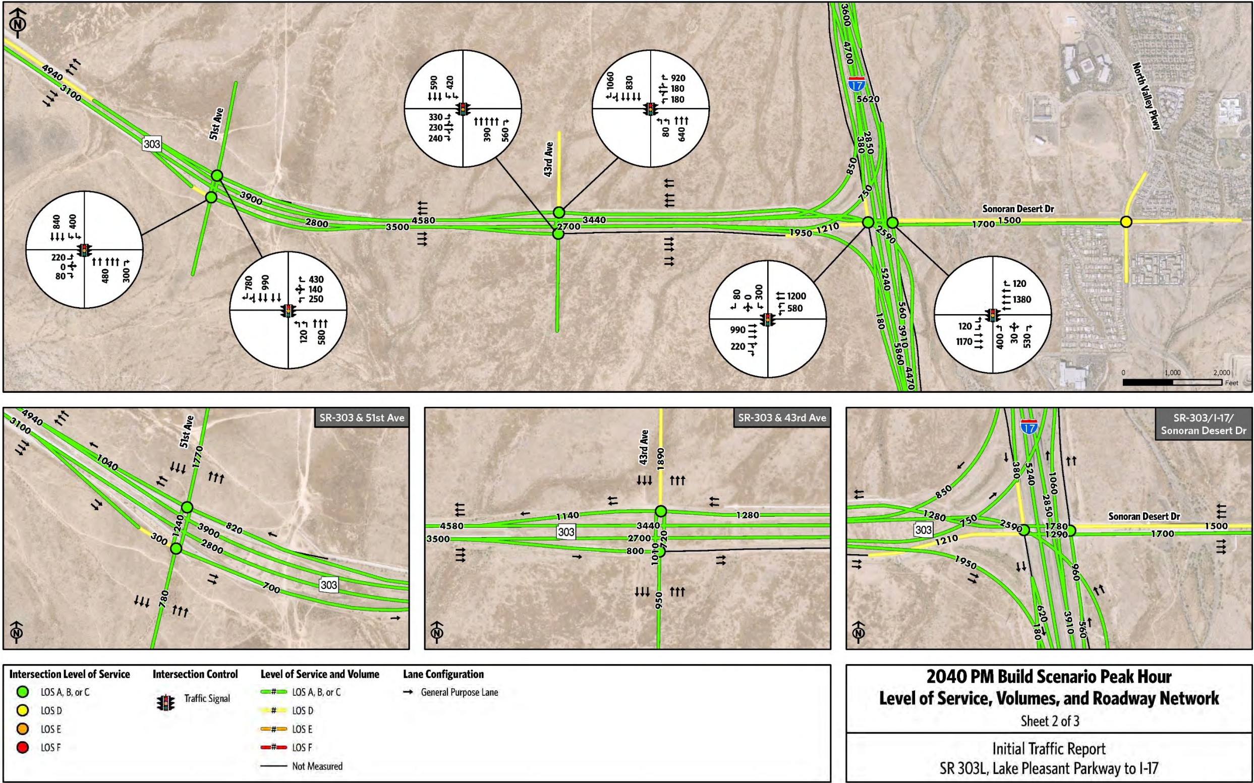
Figure 4-20: Year 2040 Build PM Peak Hour - Traffic Volumes, Lanes, & LOS (Sheet 2 of 3)
