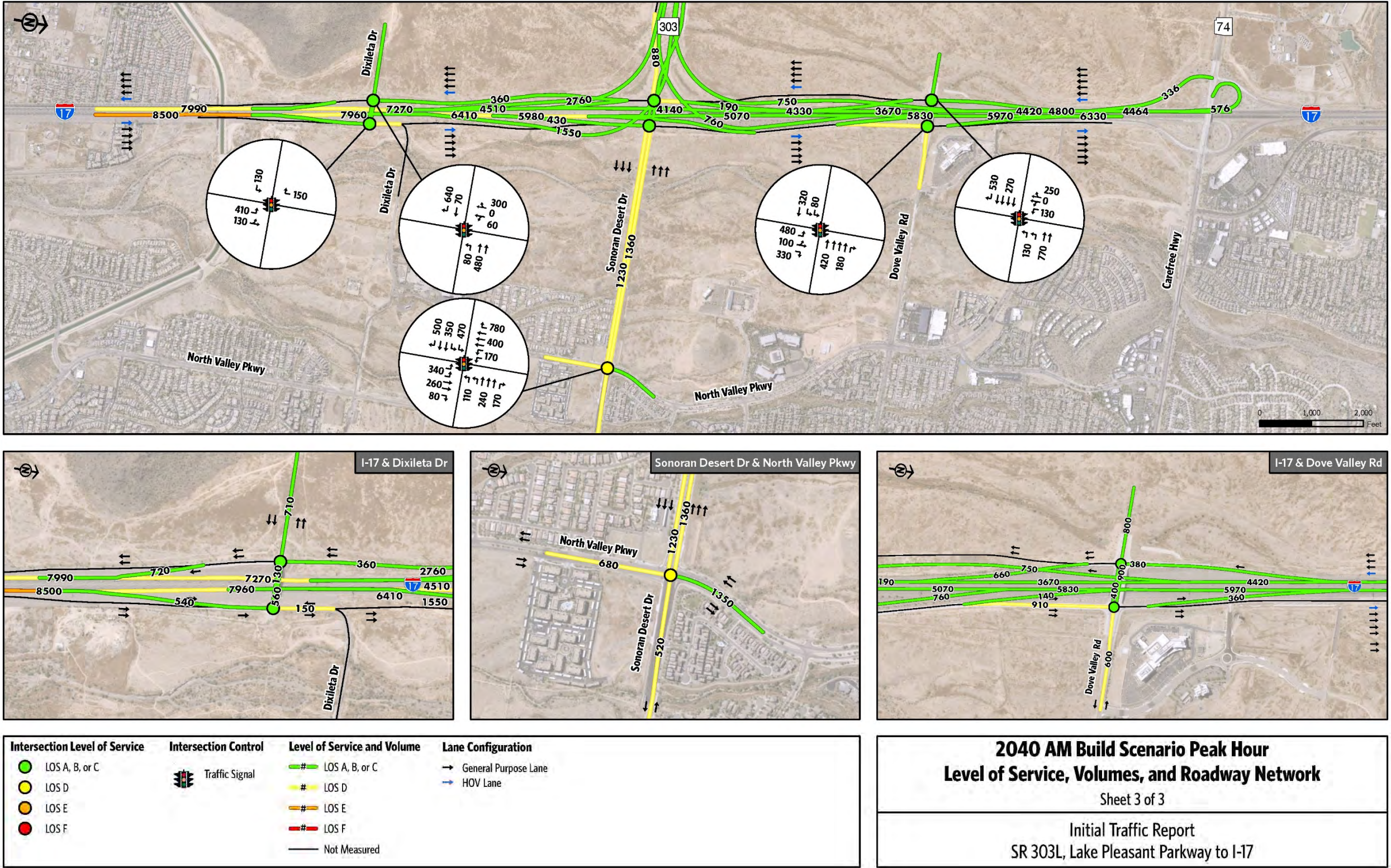
Figure 4-18: Year 2040 Build AM Peak Hour - Traffic Volumes, Lanes, & LOS (Sheet 3 of 3)
