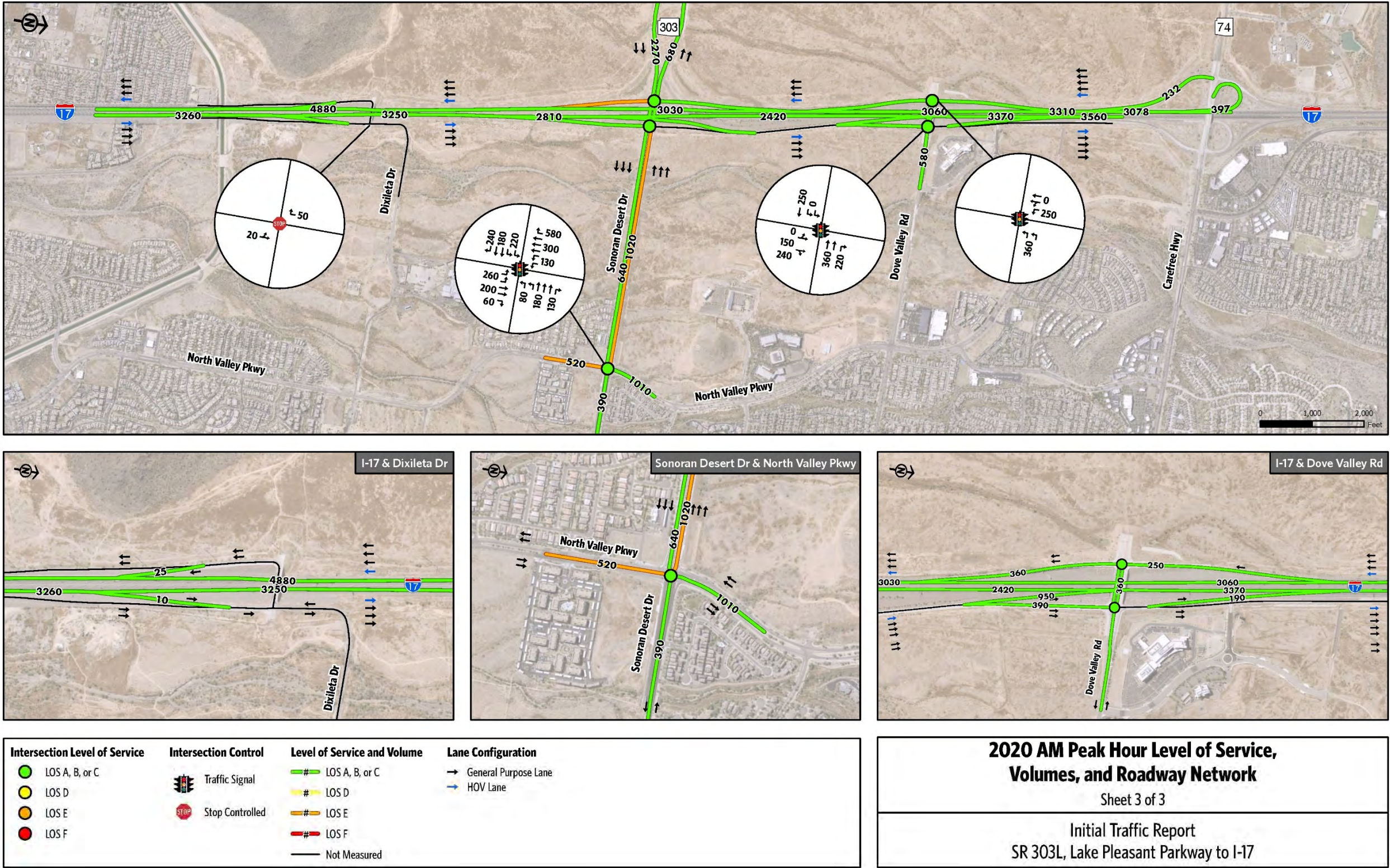
Figure 4-3: Year 2020 Existing AM Peak Hour– Traffic Volumes, Lanes, & LOS (Sheet 3 of 3)
