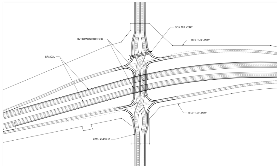
Figure 4-9: Diverging Diamond Interchange
