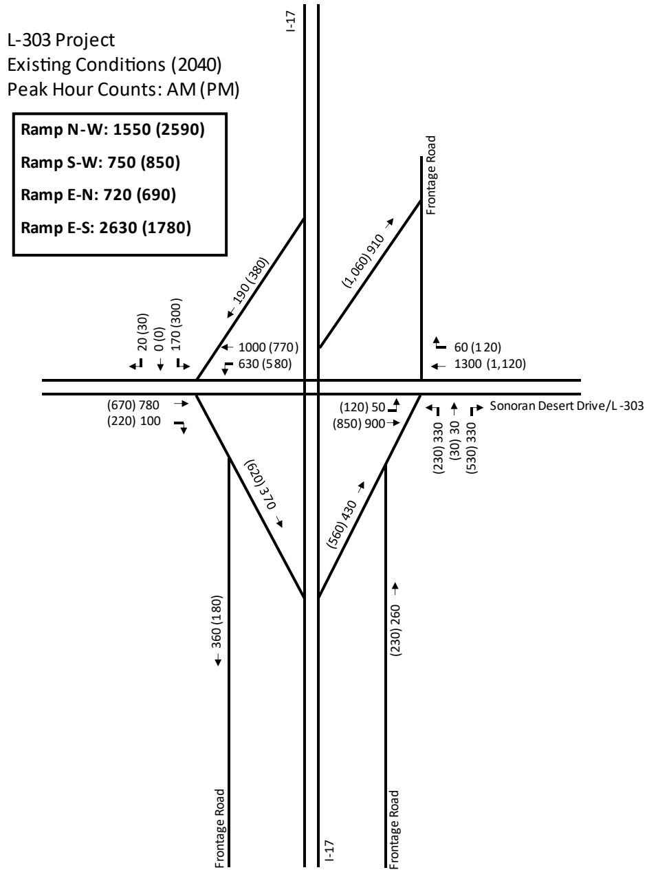
Figure 14: Loop 303 and I-17 Interchange Forecast
