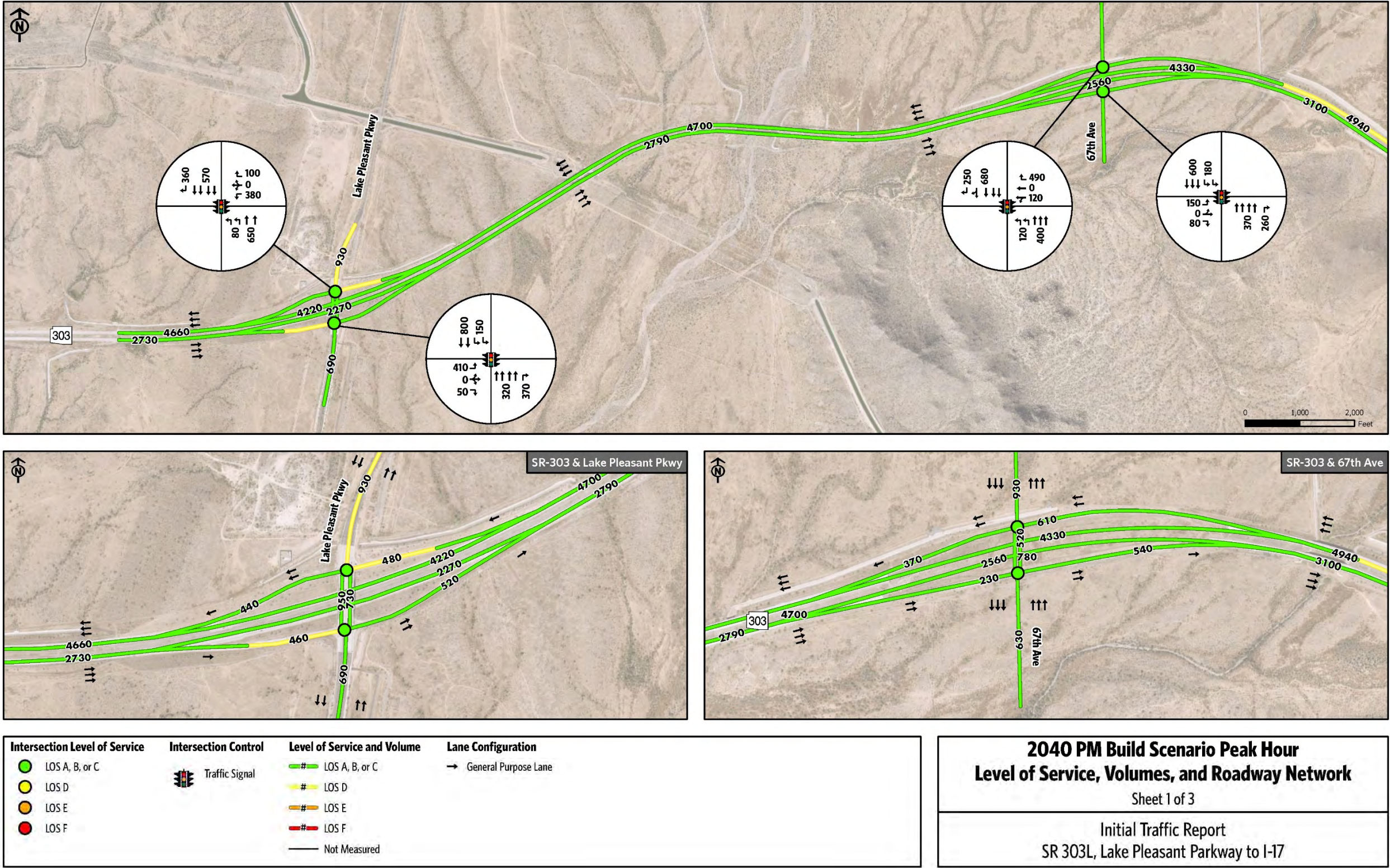
Figure 4-19: Year 2040 Build PM Peak Hour - Traffic Volumes, Lanes, & LOS (Sheet 1 of 3)
