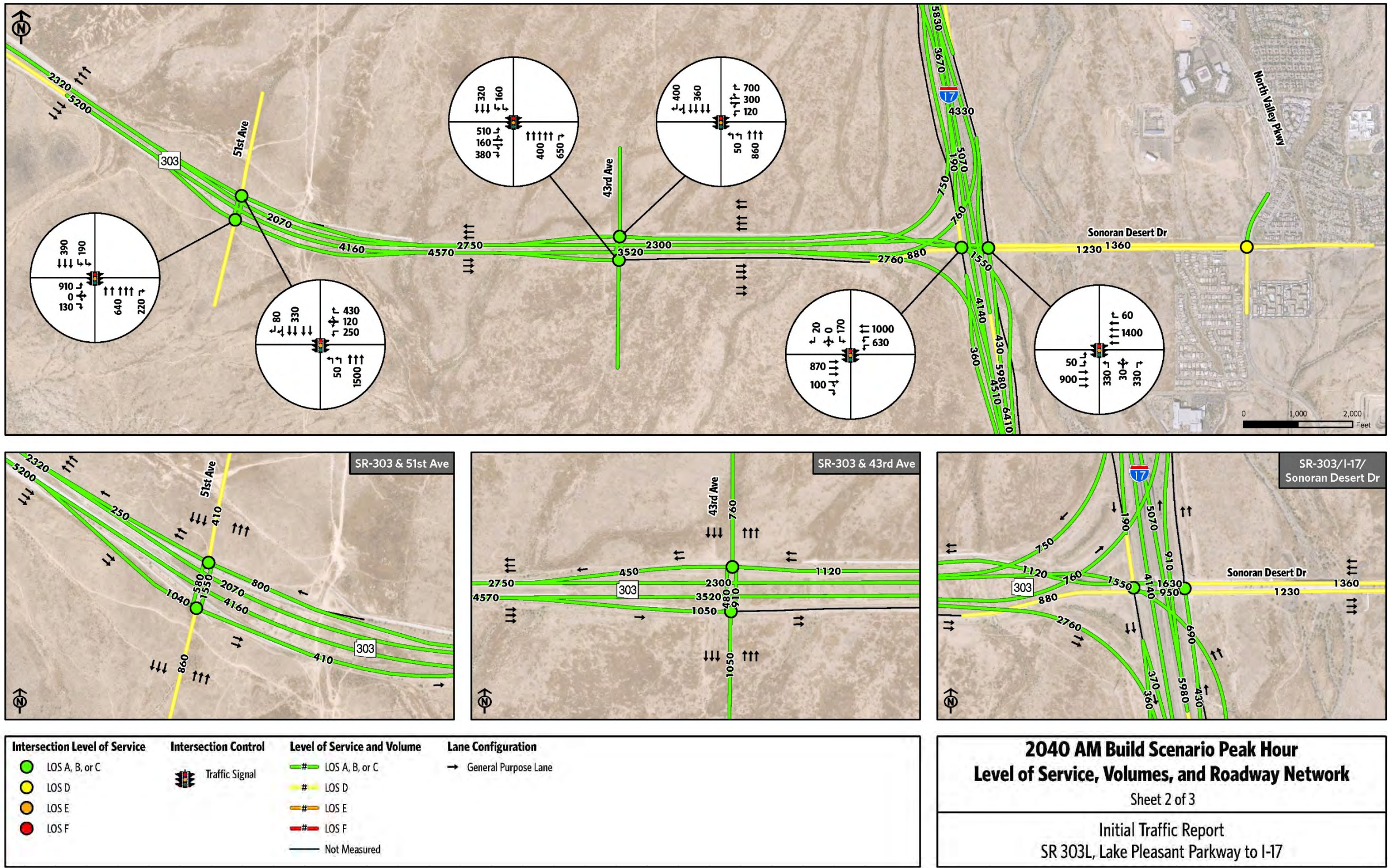
Figure 4-17: Year 2040 Build AM Peak Hour - Traffic Volumes, Lanes, & LOS (Sheet 2 of 3)
