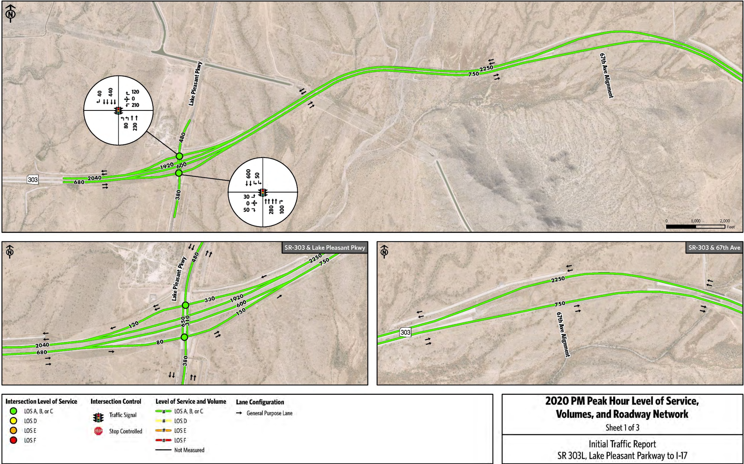
Figure 4-4: Year 2020 Existing PM Peak Hour– Traffic Volumes, Lanes, & LOS (Sheet 1 of 3)
