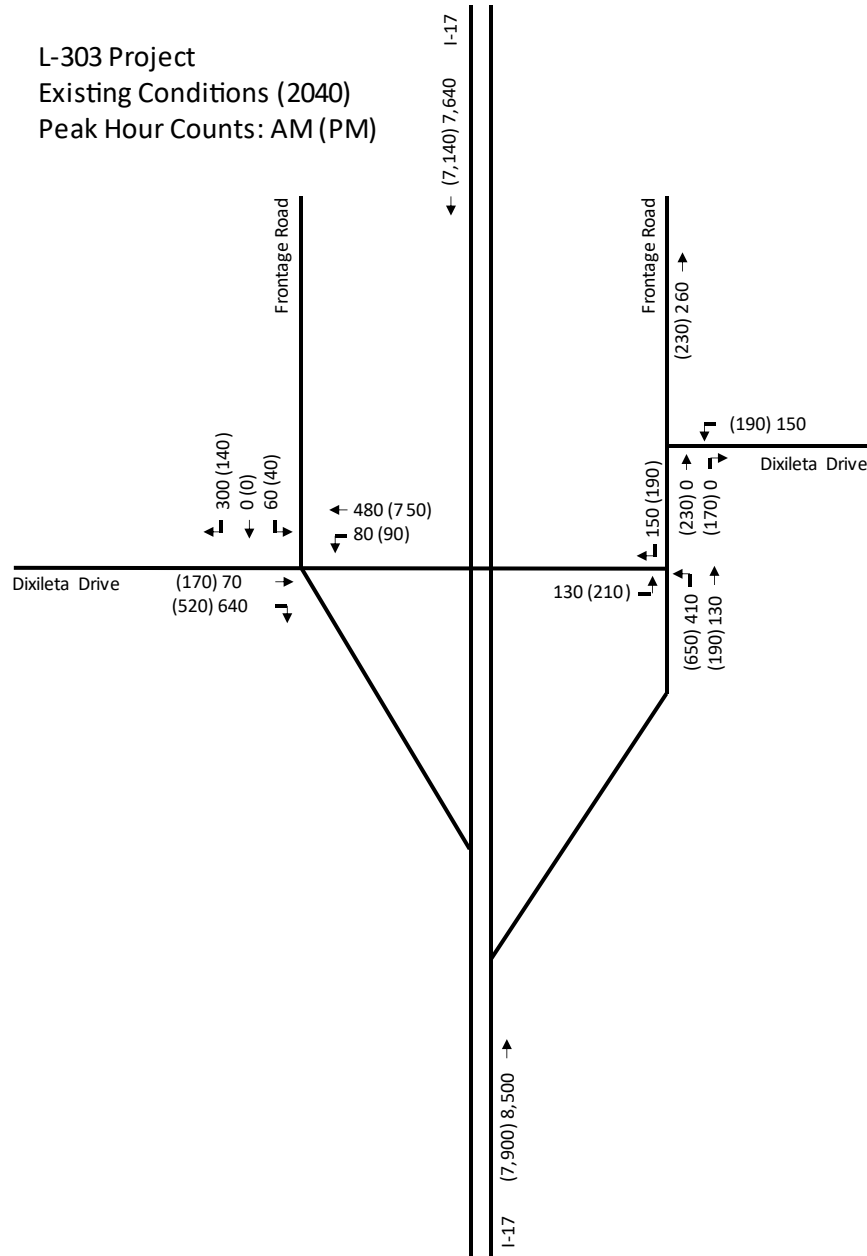
Figure 17: Dixileta Drive and I-17 Interchange Forecast
