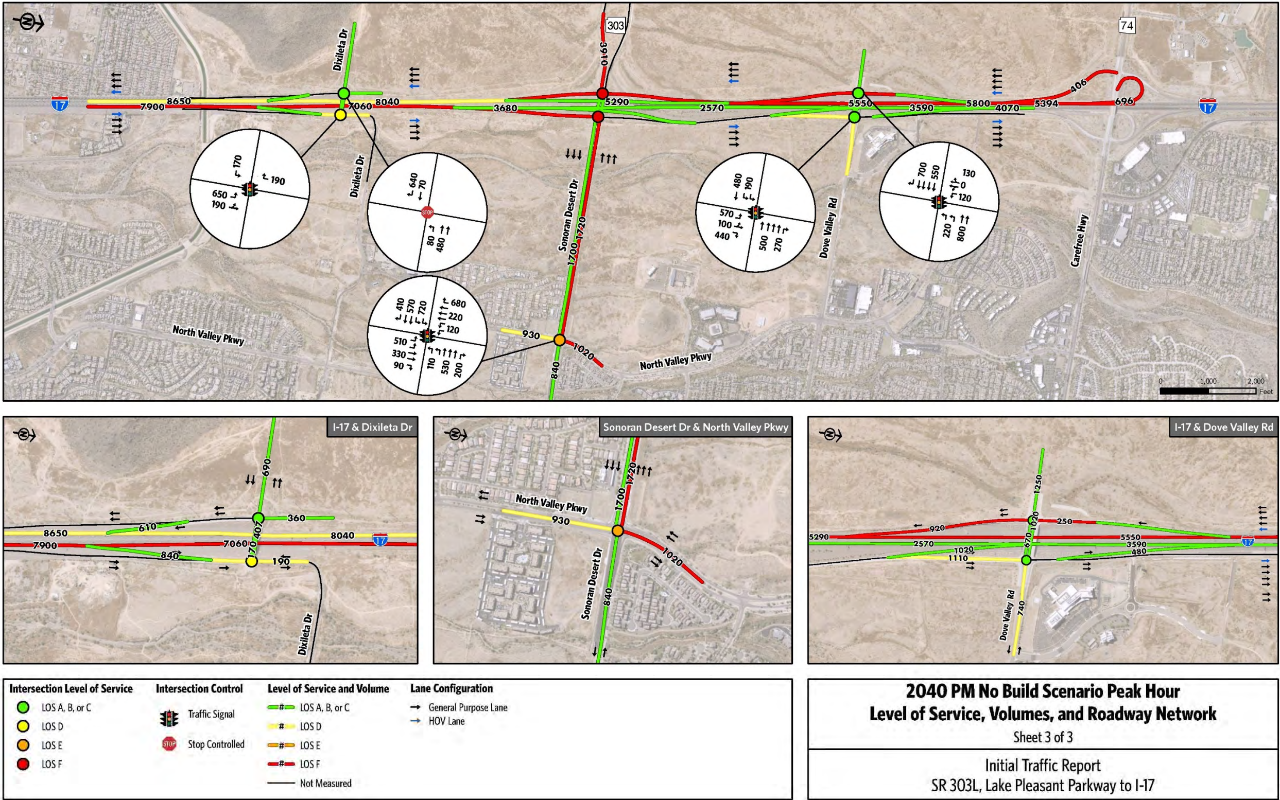
Figure 4-15: Year 2040 No Build PM Peak Hour - Traffic Volumes, Lanes, & LOS (Sheet 3 of 3)
