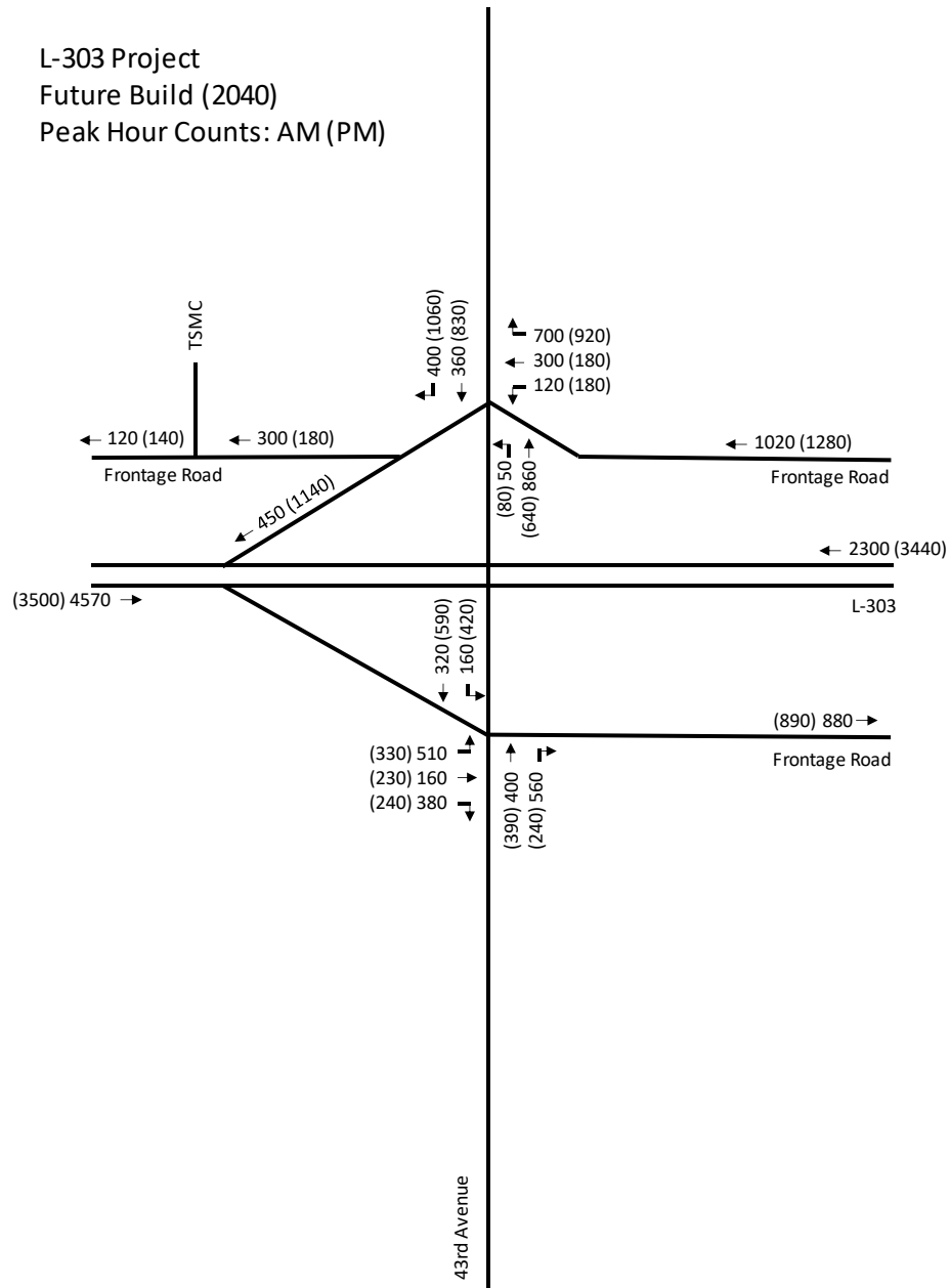
Figure 13: Loop 303 and 43rd Avenue Interchange Forecast
