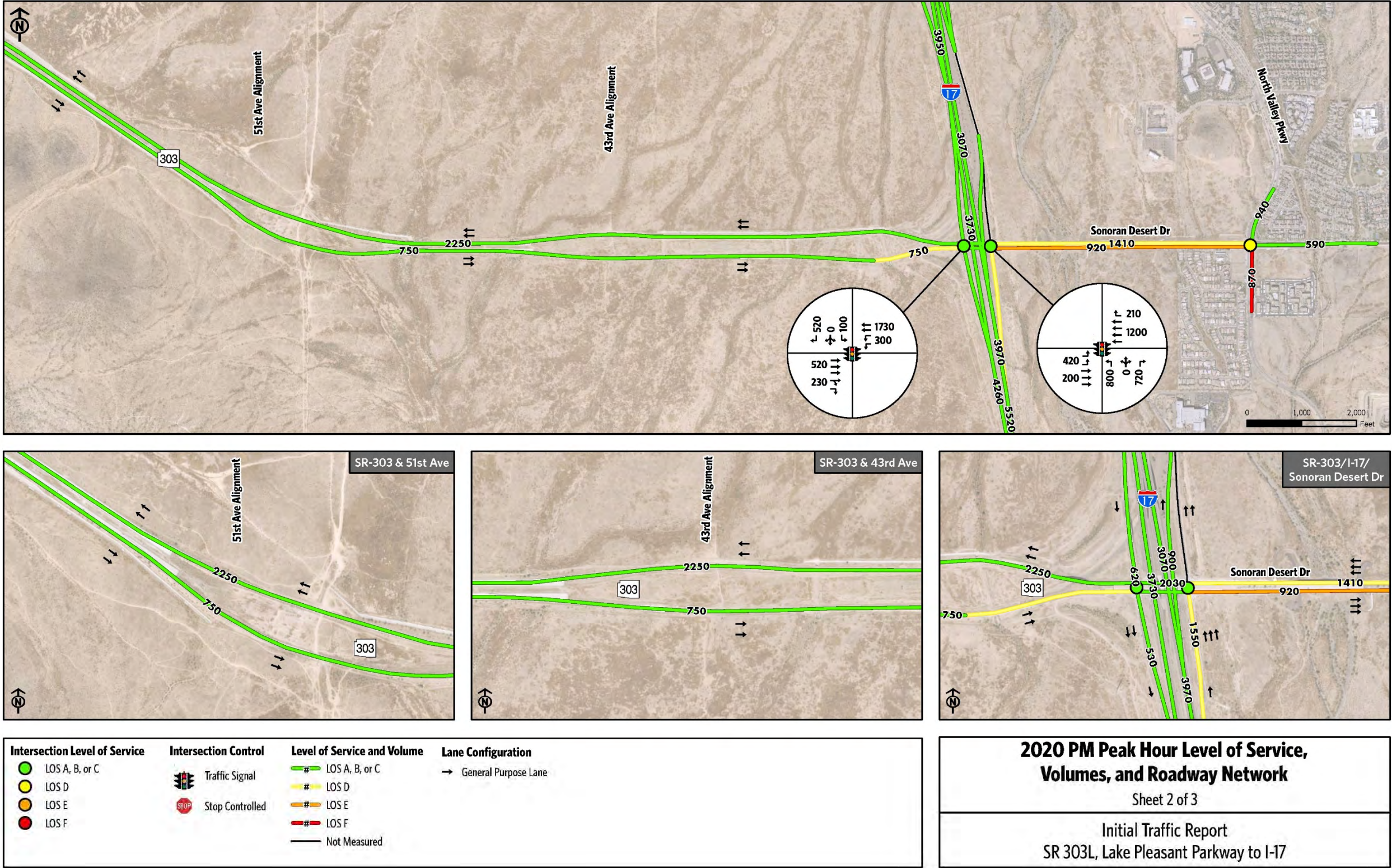
Figure 4-5: Year 2020 Existing PM Peak Hour– Traffic Volumes, Lanes, & LOS (Sheet 2 of 3)
