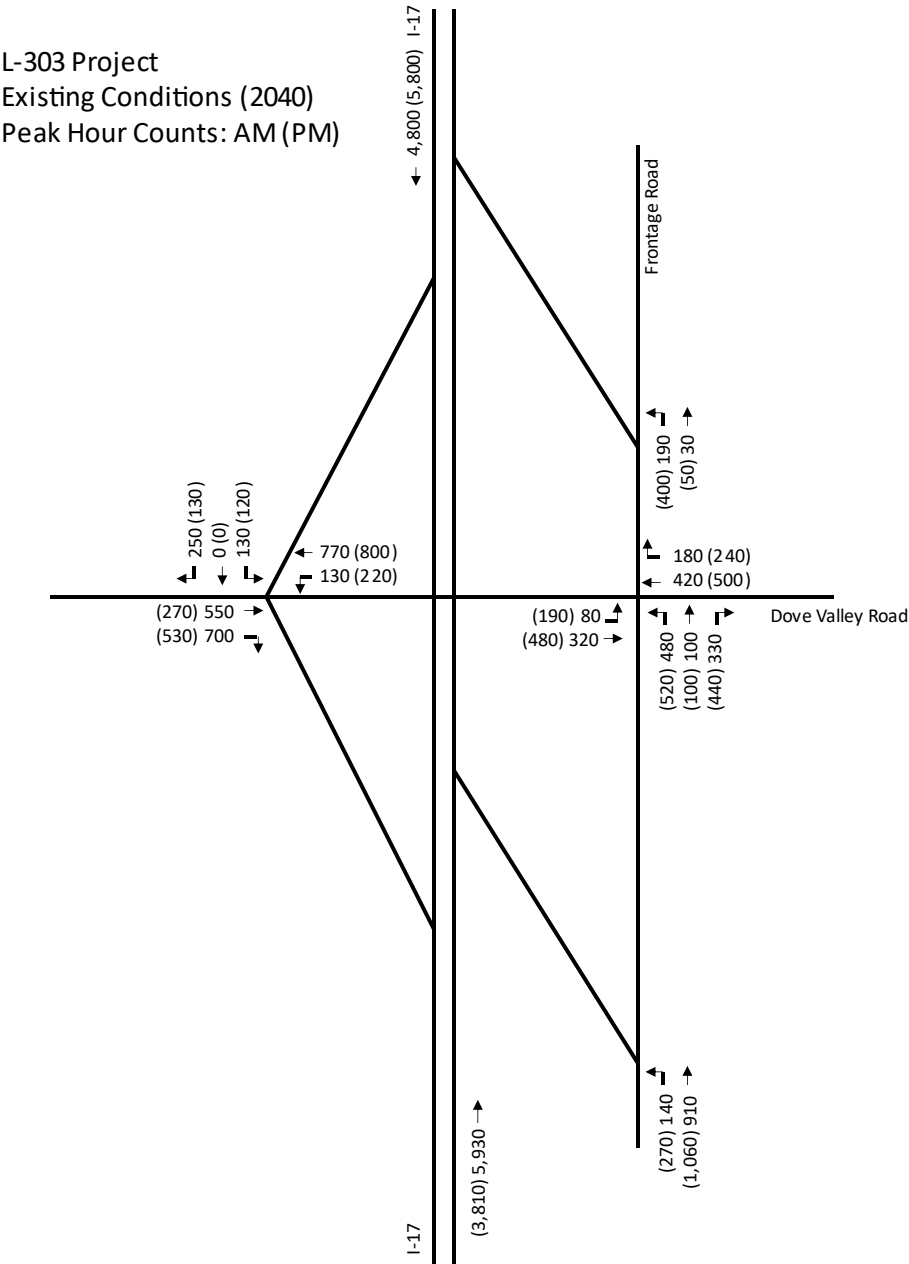
Figure 16: Dove Valley Road and I-17 Interchange Forecast
