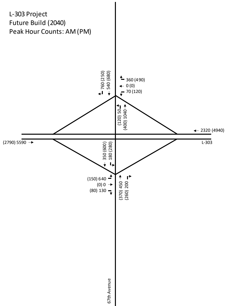
Figure 11: Loop 303 and 67th Avenue Interchange Forecast
