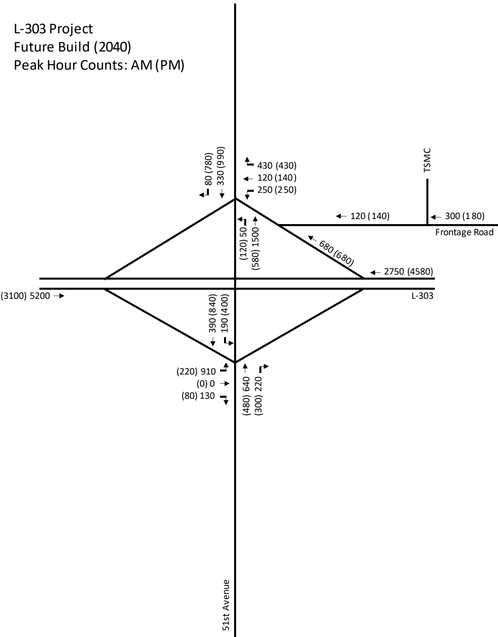
Figure 12: Loop 303 and 51st Avenue Interchange Forecast
