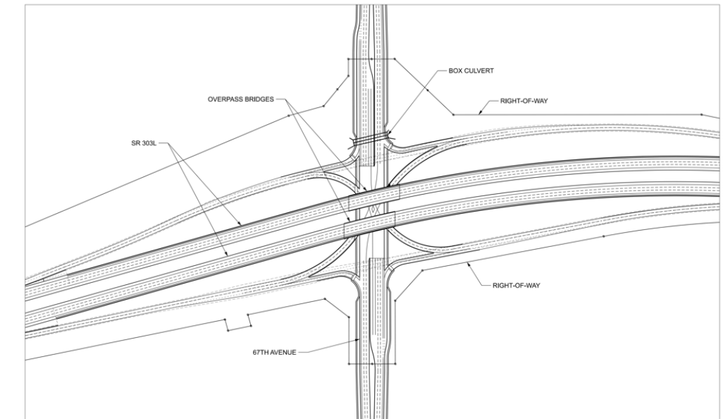
Figure 4-8: Single-Point Urban Interchange
