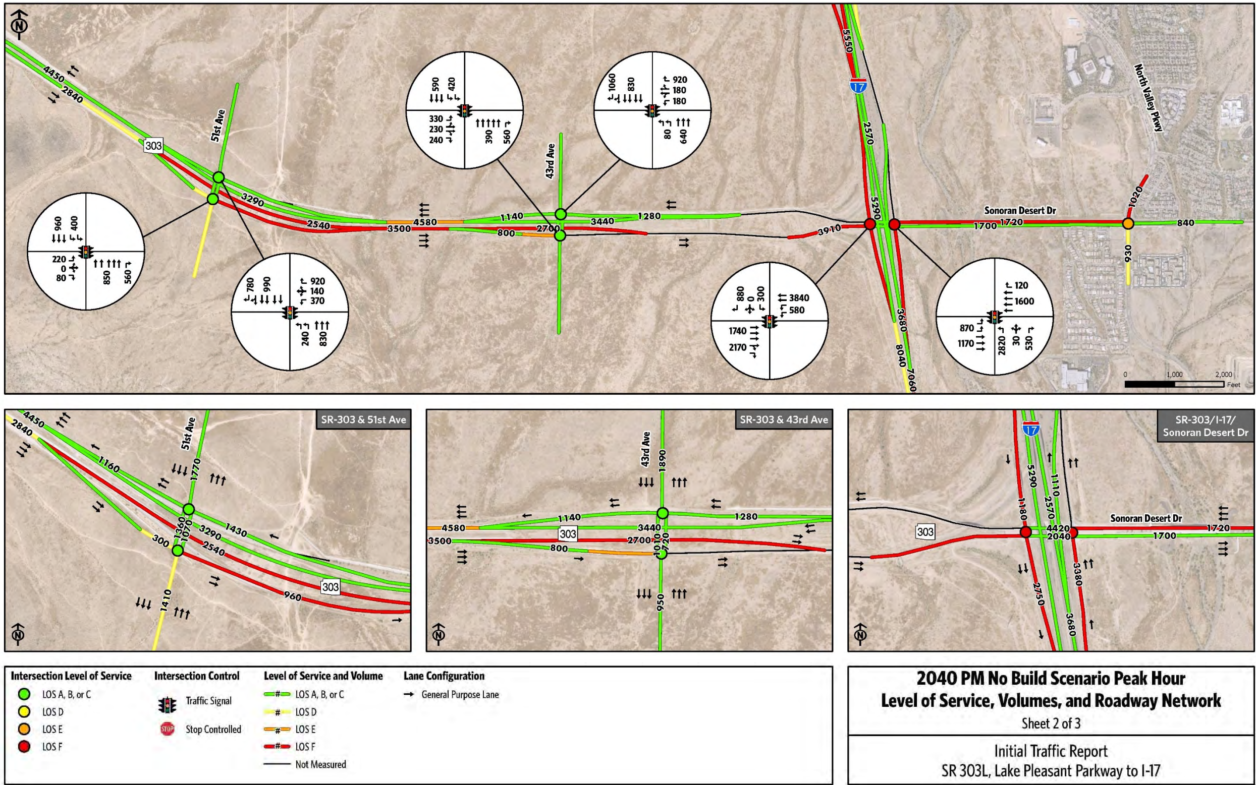
Figure 4-14: Year 2040 No Build Peak Hour PM - Traffic Volumes, Lanes, & LOS (Sheet 2 of 3)
