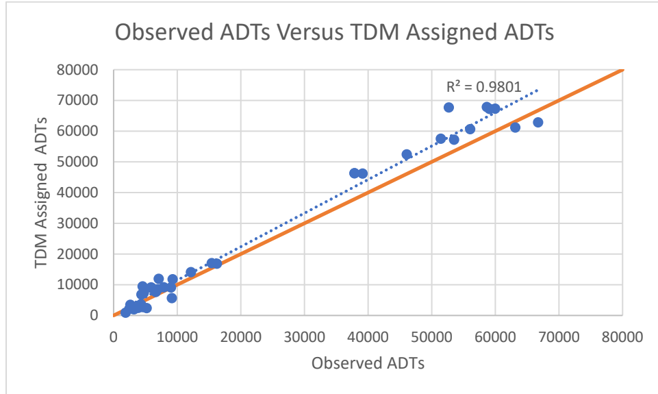
Figure 3: Observed AADTs Versus Modeled AADTs Goodness of Fit
