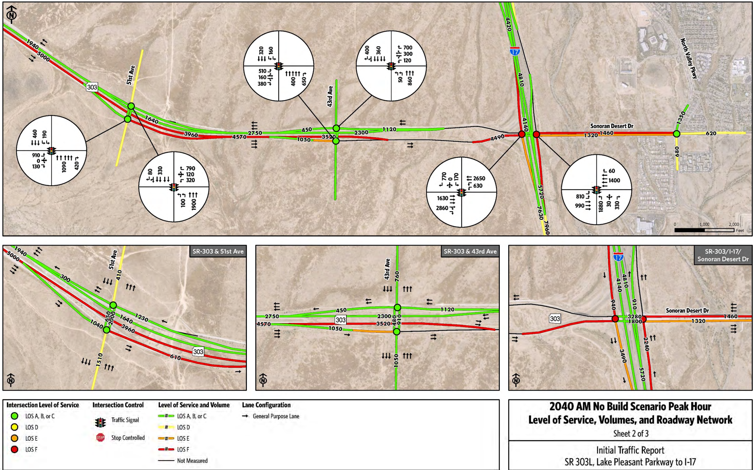
Figure 4-11: Year 2040 No Build AM Peak Hour - Traffic Volumes, Lanes, & LOS (Sheet 2 of 3)
